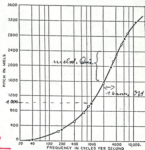
Fig. 10. Relation between pitch and the frequency of pure tones 40 db above threshold (STEVENS and VOLKMANN [53]).
