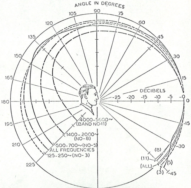
Fig. 10. Spatial distribution of pressures in certain frequency bands of speech, in a vertical plane through the lips of the speaker (after Dunn and Farnsworth).
