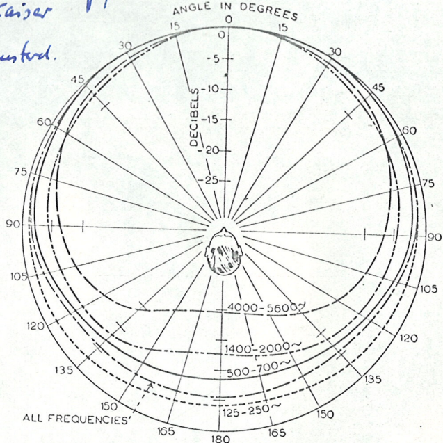
Fig. 9. Spatial distribution of pressures in certain frequency bands of speech, in a horizontal plane through the lips of the speaker (after Dunn and Farnsworth).
