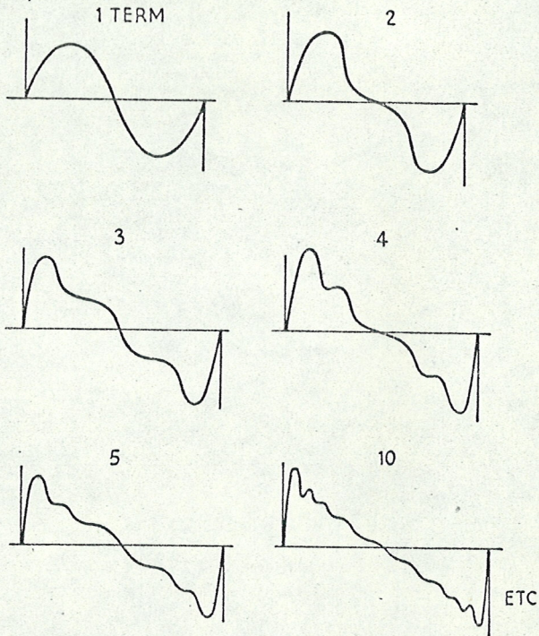
FIG. 27. FORMATION OF A SAWTOOTH WAVE
