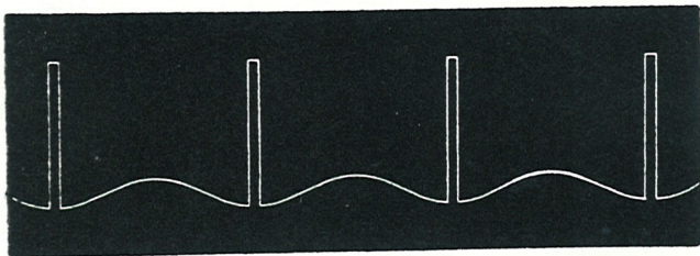
Fig. 1. Elimination of components. a. Periodic impulse of width \frac{2\pi}{20} . b. Periodic
